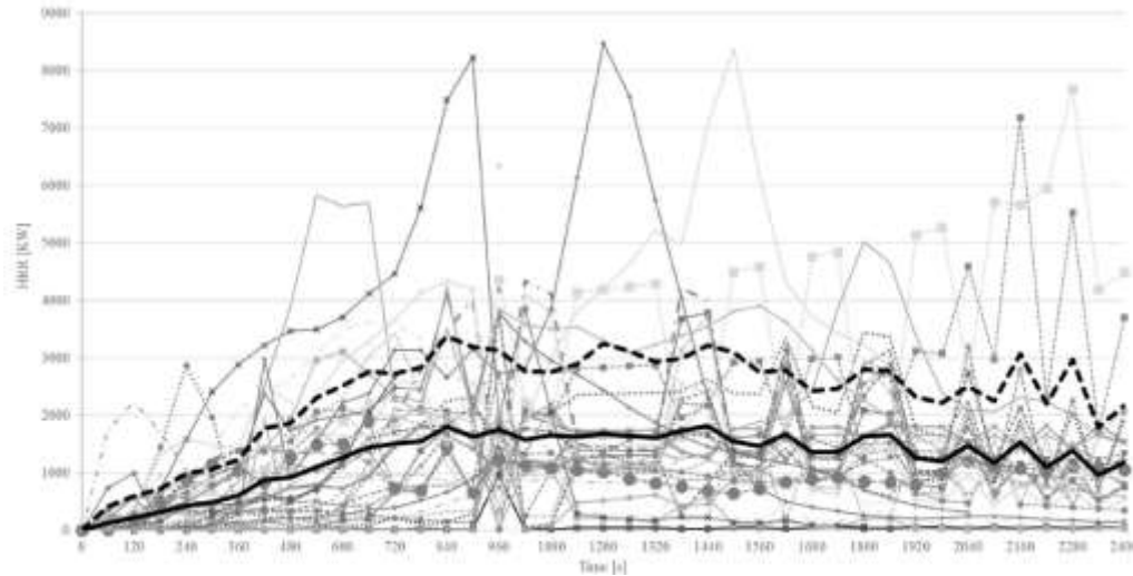
Figure 1 - Change in heat release rate of 44 full-scale vehicle fires [14]
