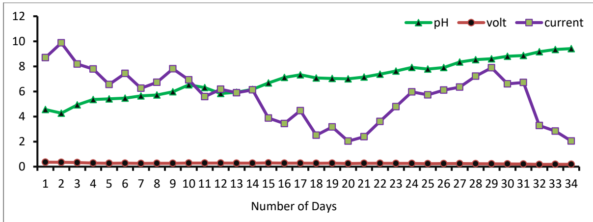
Figure 4: Graph of pH, voltage and current readings from Table 2
